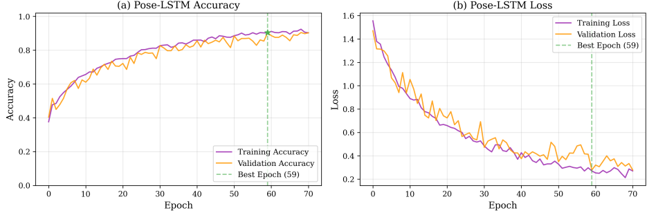
Fig. 7 Pose-LSTM Training Curves
